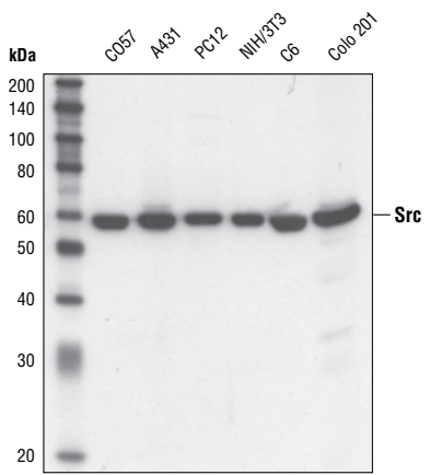
Western blot analysis of cell extracts from various cell lines using Src (L4A1) Mouse mAb.
