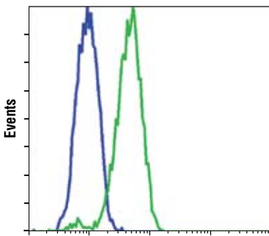
Phospho-Akt (Ser473) (Alexa Fluor® 488) Flow cytometric analysis of Jurkat cells, untreated (green) or LY294002 and wortmannin treated (blue) using Phospho-Akt (Ser473) (193H12) Rabbit mAb (Alexa Fluor® 488 conjugate).
