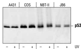
Western blot analysis of extracts from A431, COS, NBT-II and JB6 cells, untreated or UV-treated, using p53 (1C12) Mouse mAb.
