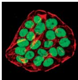
Confocal immunofluorescent analysis of HT-29 cells using p53 (1C12) Mouse mAb (green). Actin filaments have been labeled with DY-554 phalloidin (red).
