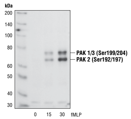
Western blot analysis of extracts from guinea pig neutrophils stimulated with iMLP (1 \mu M) for the indicated times, using Phospho-PAK1 (Ser199/204)/PAK2 (Ser192/197) Antibody.
