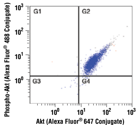
Flow cytometric analysis of Jurkat cells, untreated (left) or or treated with LY294002, wortmannin and U0126 (right), using Akt (5G3) Mouse mAb (Alexa Fluor ® 647 Conjugate) and Phospho-Akt (Ser473) (D9E) Rabbit mAb (Alexa Fluor ® 488Conjugate) #4071.
