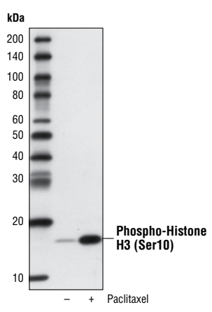
Western blot analysis of extracts from HeLa cells, untreated or treated with Paclitaxel #9807, using Phospho-Histone H3 (Ser10) (D2C8) Rabbit mAb (Biotinylated) #3642 and Streptavidin-HRP #3999 for detection.
